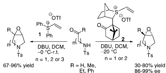
Scheme 1. Vinyl Sulfonium Salt Mediated Epoxy-Annulation Reaction of Achiral \alpha -, \beta -, and \gamma -Amido Aldehydes/Ketones
