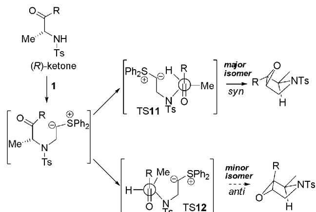
Scheme 2. Proposed Model for Substrate-Controlled Annulation Reaction
