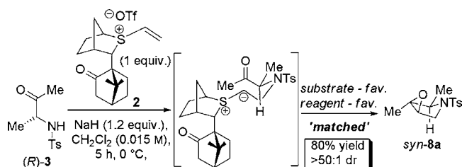
Scheme 3. Proposed Model for “Matched” Reaction of ( R )-Amido Methyl-Ketone ( R )- 3 with Chiral Vinyl Sulfonium Salt 2 (Method B)
