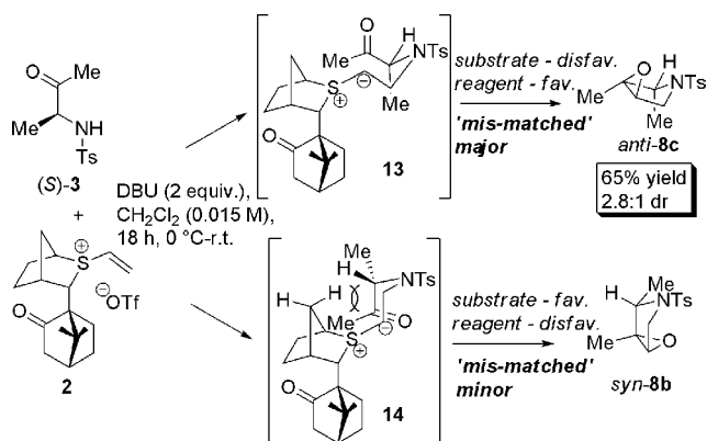
Scheme 4. Proposed Model for “Mis-Matched” Reaction of ( S )-Amido Methyl-Ketone ( S )- 3 with Chiral Vinyl Sulfonium Salt 2 (Method C)
